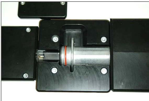
Unit under test in adapter with form fitting contour
